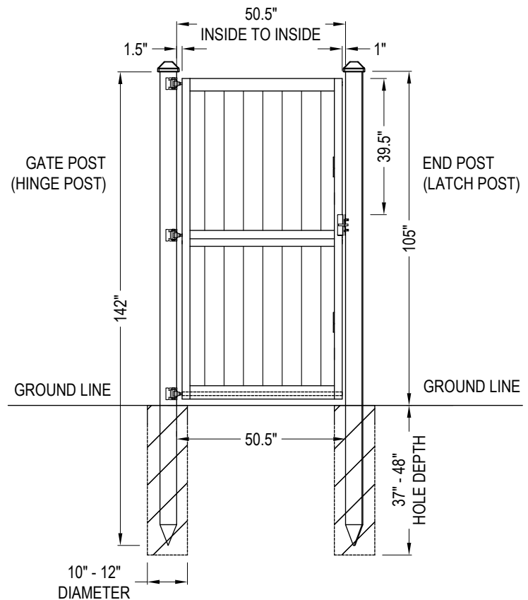
ELEVATION VIEW
