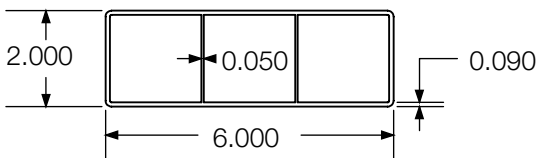
2" x 6" Rail
