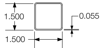
1½" x 1½" Picket
