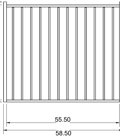
4'x60" STRAIGHT WALK GATE
